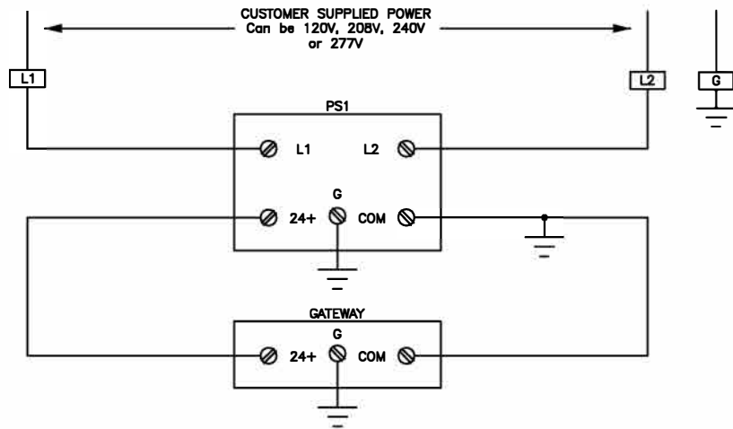
GATEWAY POWER SUPPLY WIRING
